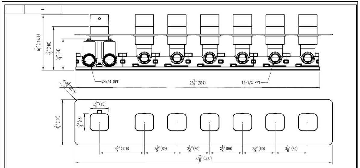
Valve Mixer
