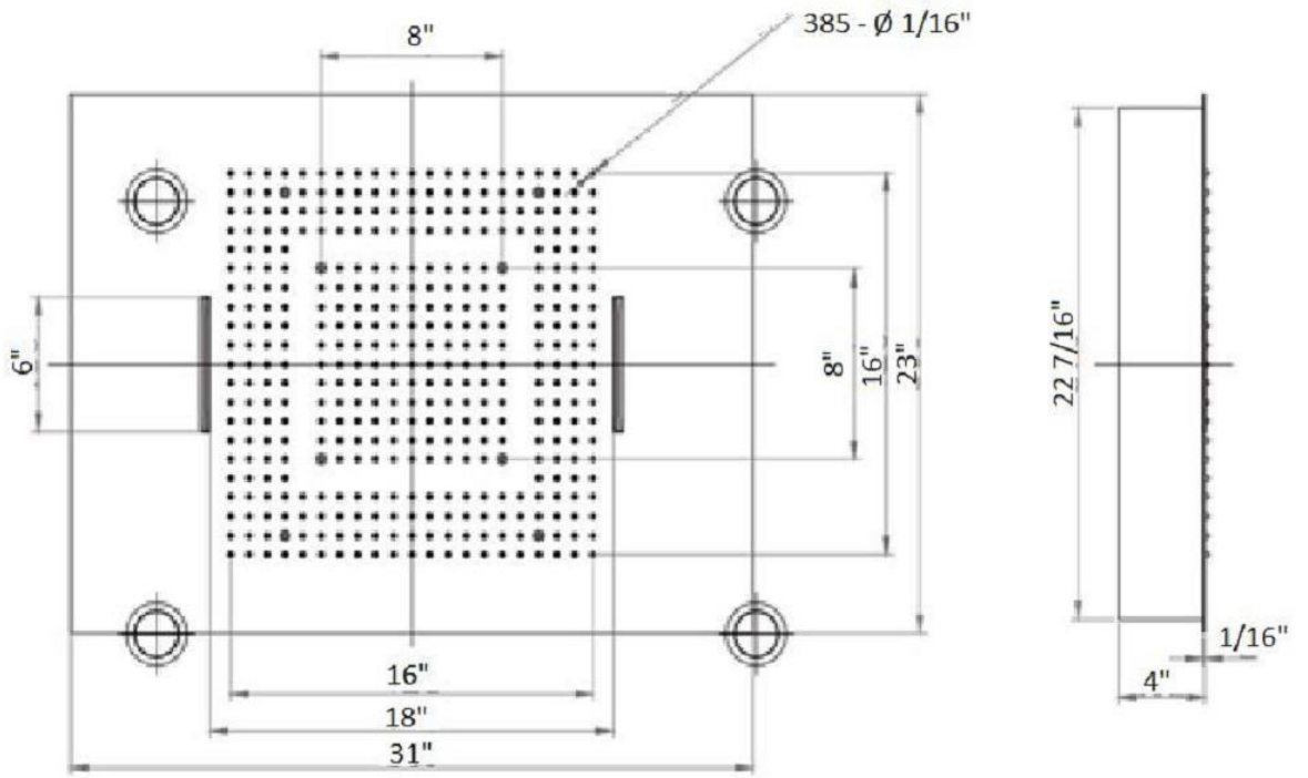
Shower Head
